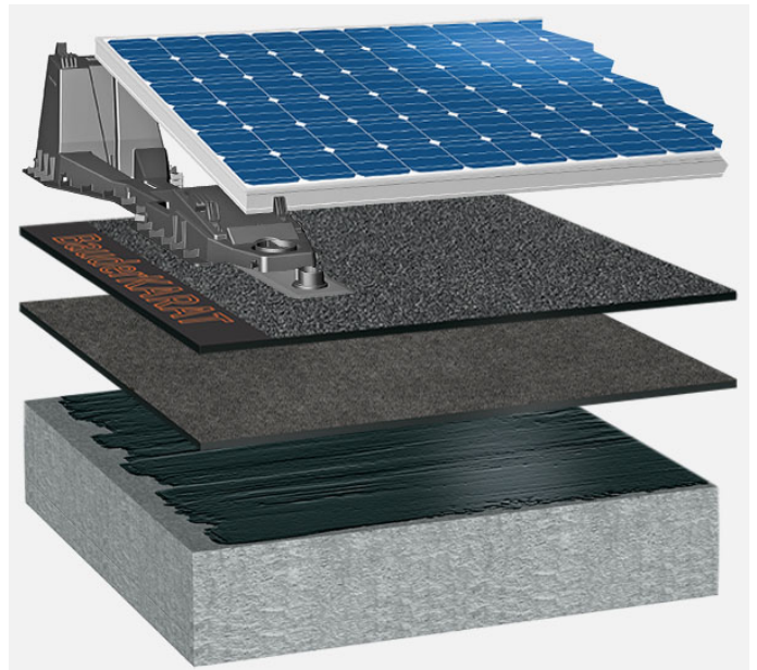
System oppbygging: BG_K_01_PVFD
