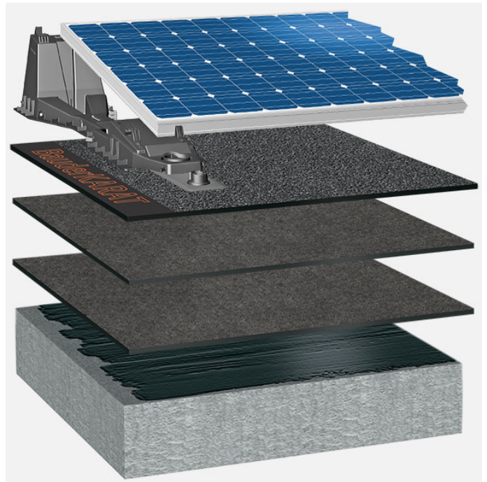
System oppbygging: BG_K_02_PVFD
