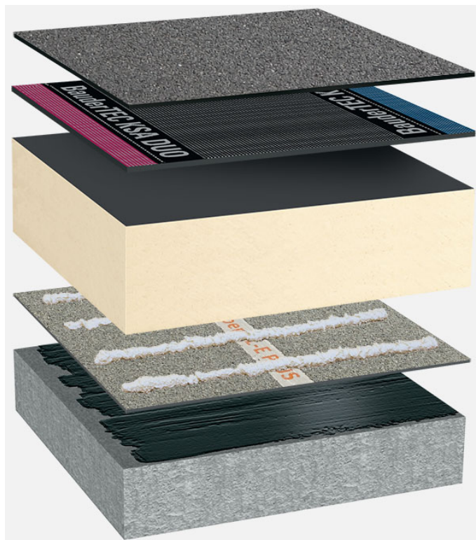
System oppbygging: BG_PIR-FA_B_01
