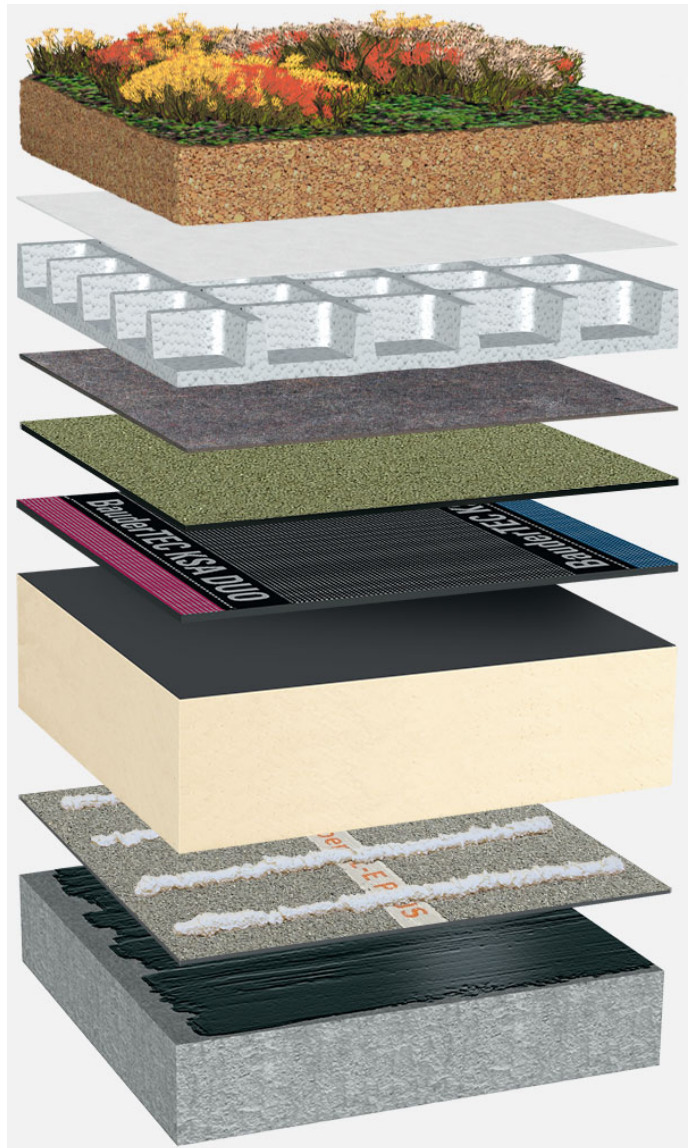
System oppbygging: BG_PIR-FA_P_01_G75
