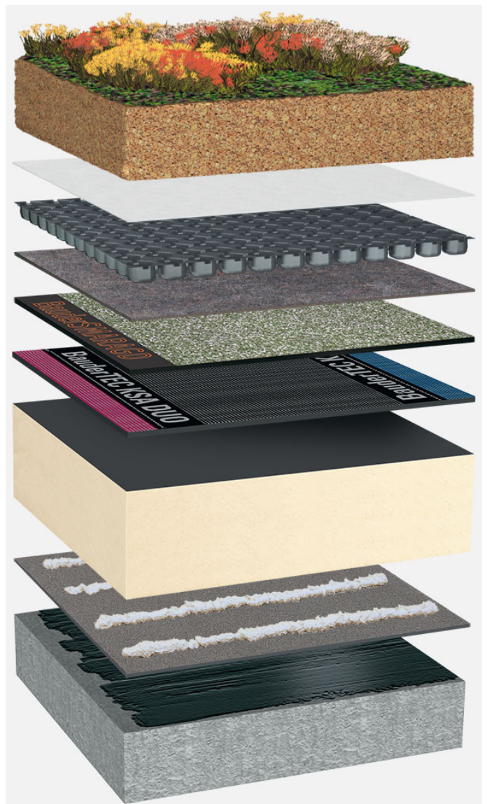
System oppbygging: BG_PIR-FA_S_01_G125
