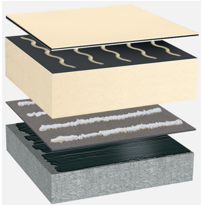
System oppbygging: BG_PIR-FA_TV_01
