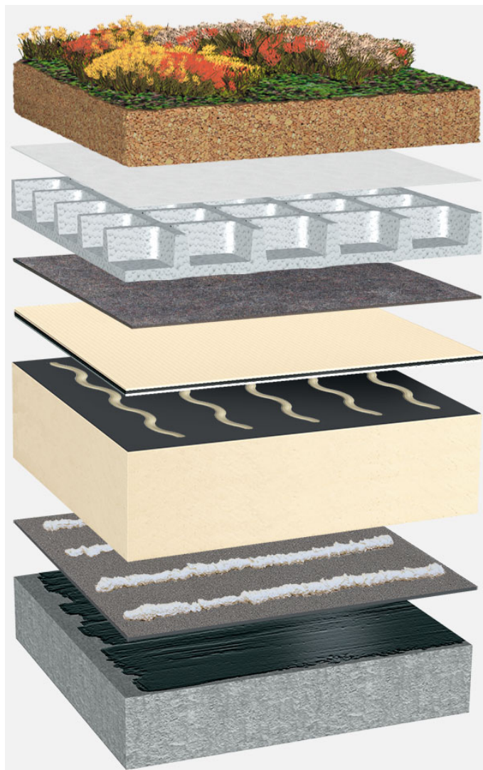
System oppbygging: BG_PIR-FA_TV_01_G75
