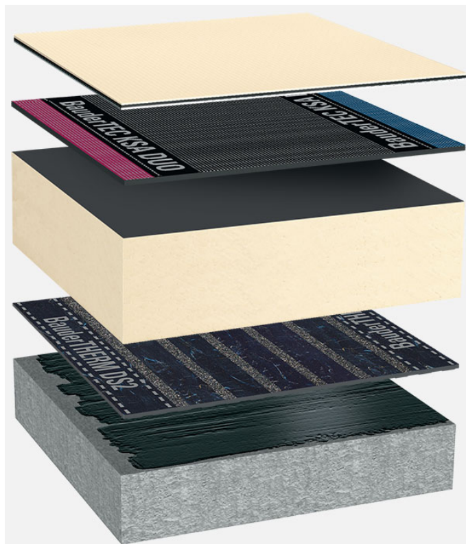
System oppbygging: BG_PIR-FA_TV_02
