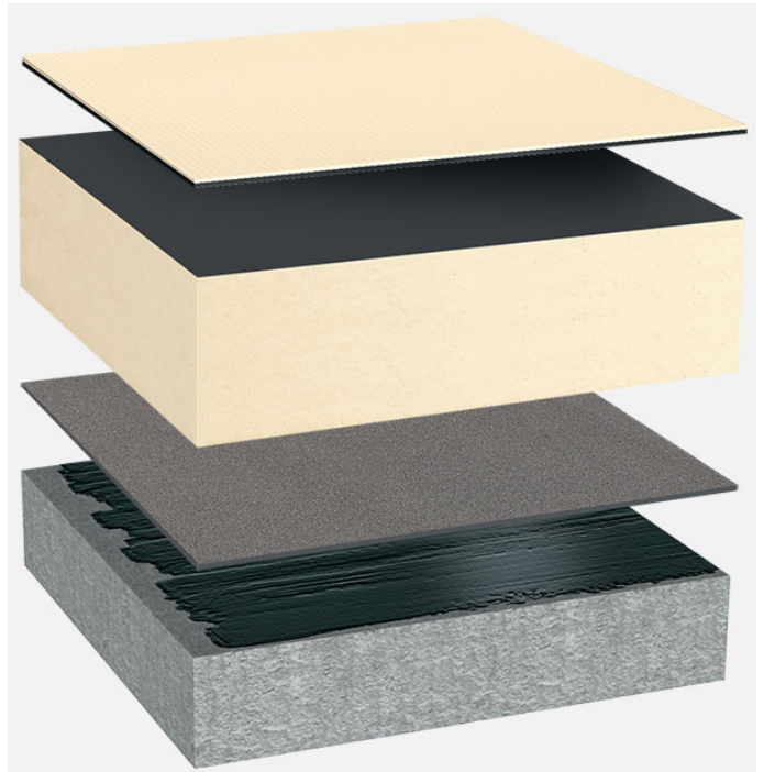
System oppbygging: BG_PIR-FA_T_01
