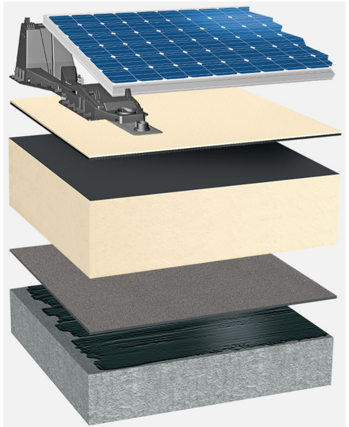
System oppbygging: BG_PIR-FA_T_01_PVFD
