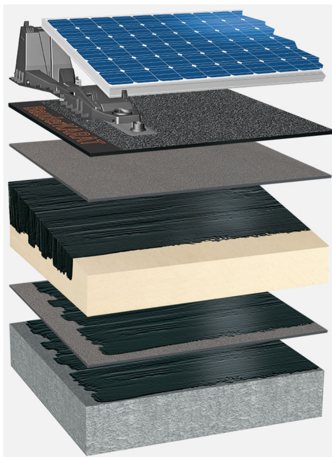
System oppbygging: BG_PIR-KP_K_01_PVFD
