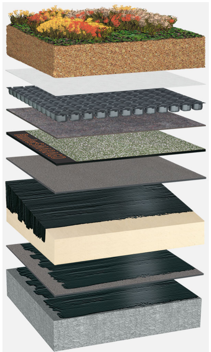
System oppbygging: BG_PIR-KP_S_01_G125
