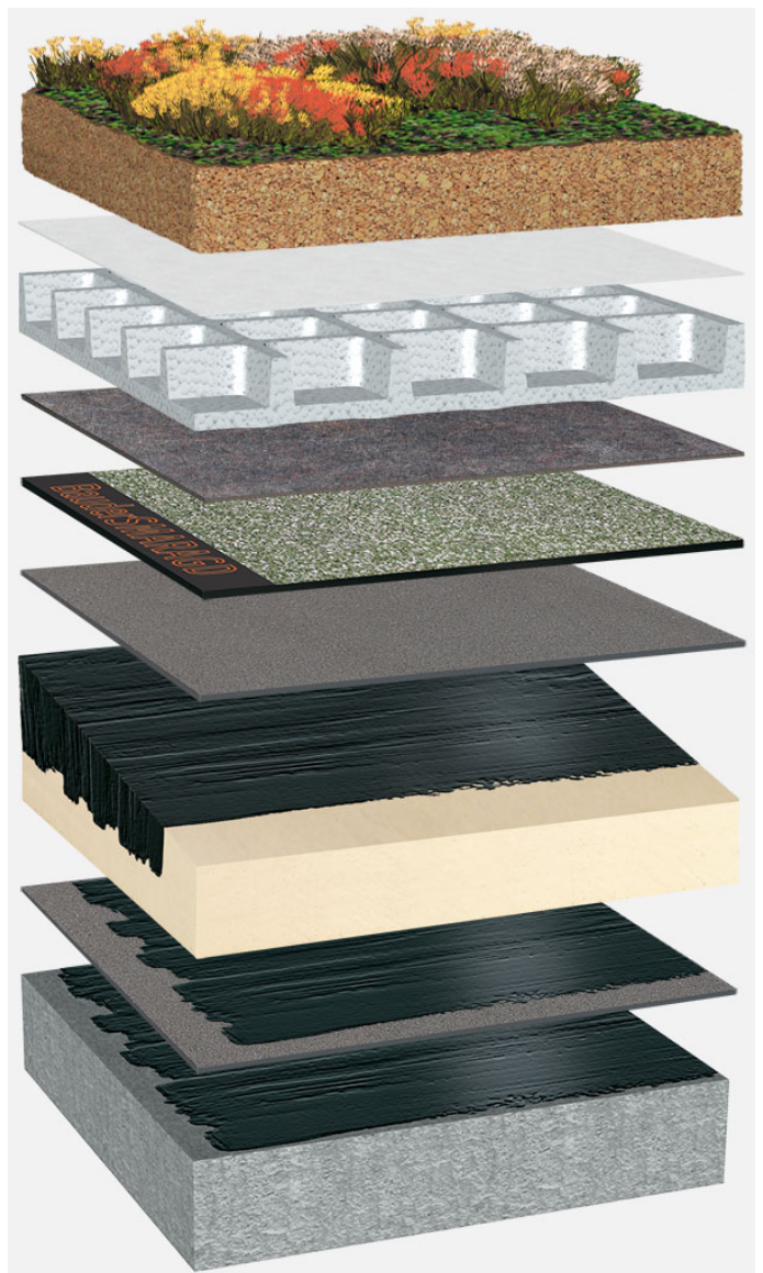
System oppbygging: BG_PIR-KP_S_01_G75
