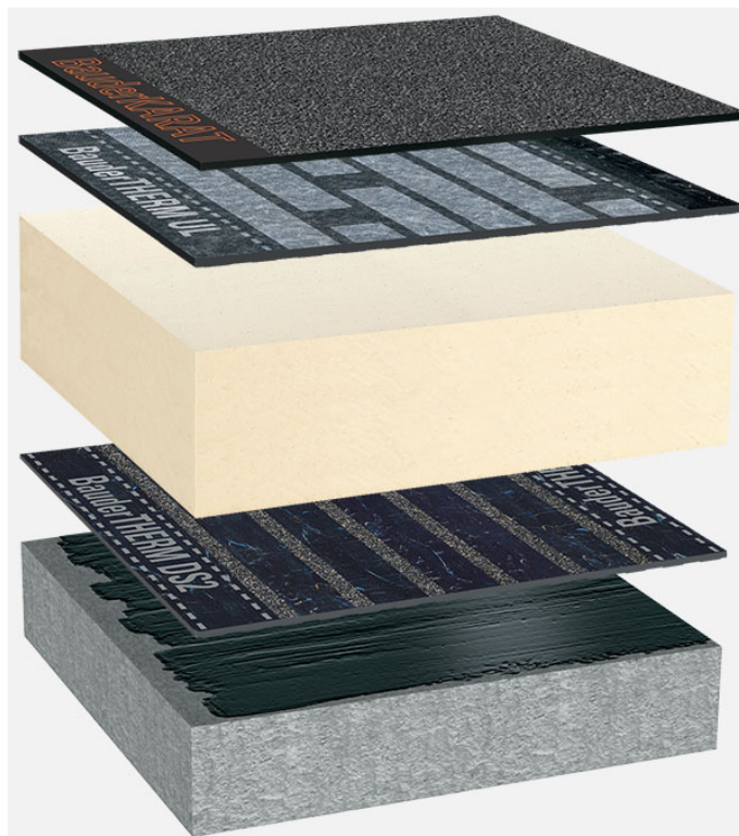
System oppbygging: BG_PIR-MF_K_01
