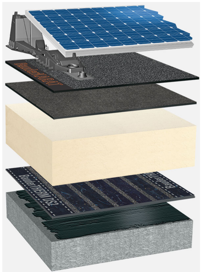
System oppbygging: BG_PIR-MF_K_01_PVFD
