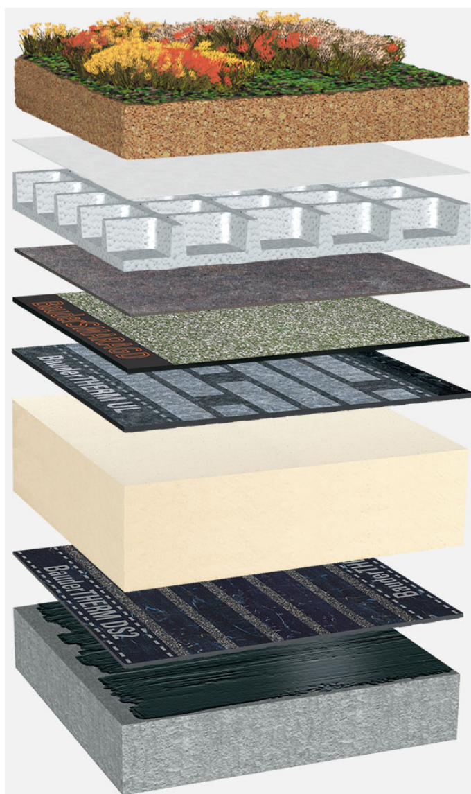
System oppbygging: BG_PIR-MF_S_01_G75
