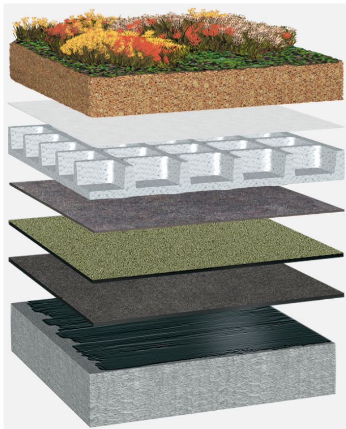
System oppbygging: BG_P_01_G75
