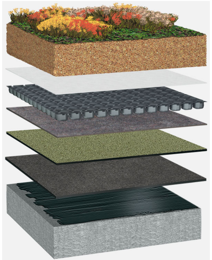
System oppbygging: BG_P_03_G125
