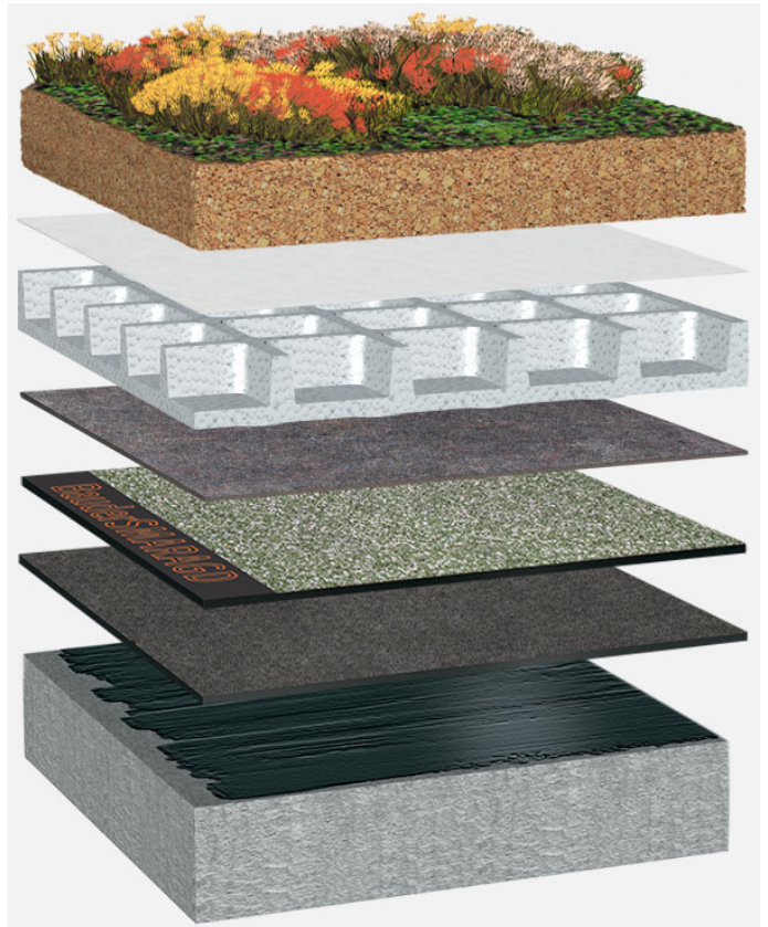
System oppbygging: BG_S_01_G75
