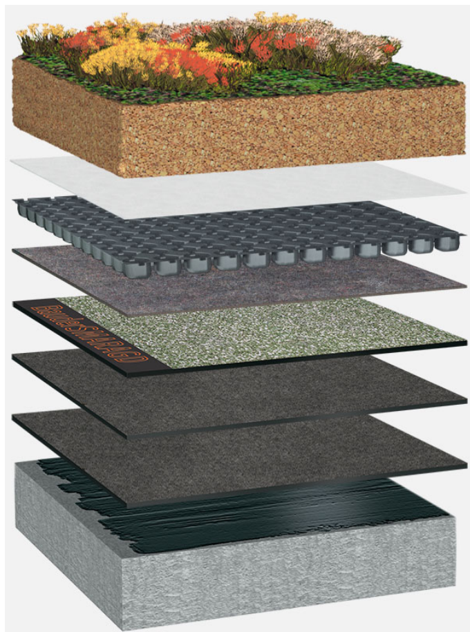
System oppbygging: BG_S_02_G125
