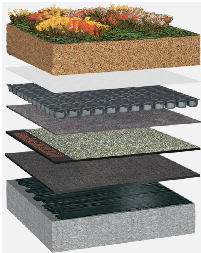
System oppbygging: BG_S_03_G125
