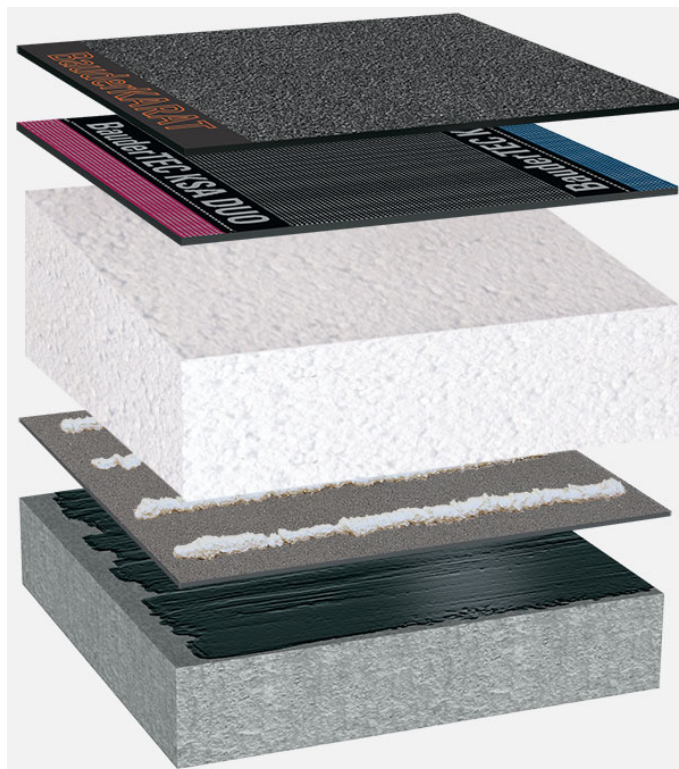
System oppbygging: BP_EPS-G_K_01
