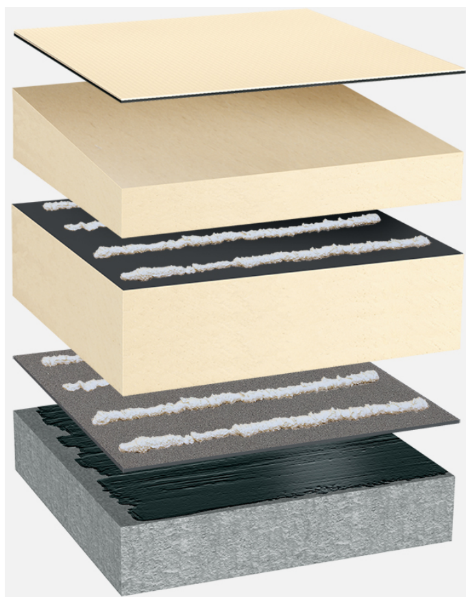
System oppbygging: BP_PIR-FA_PIR-TG_T_01
