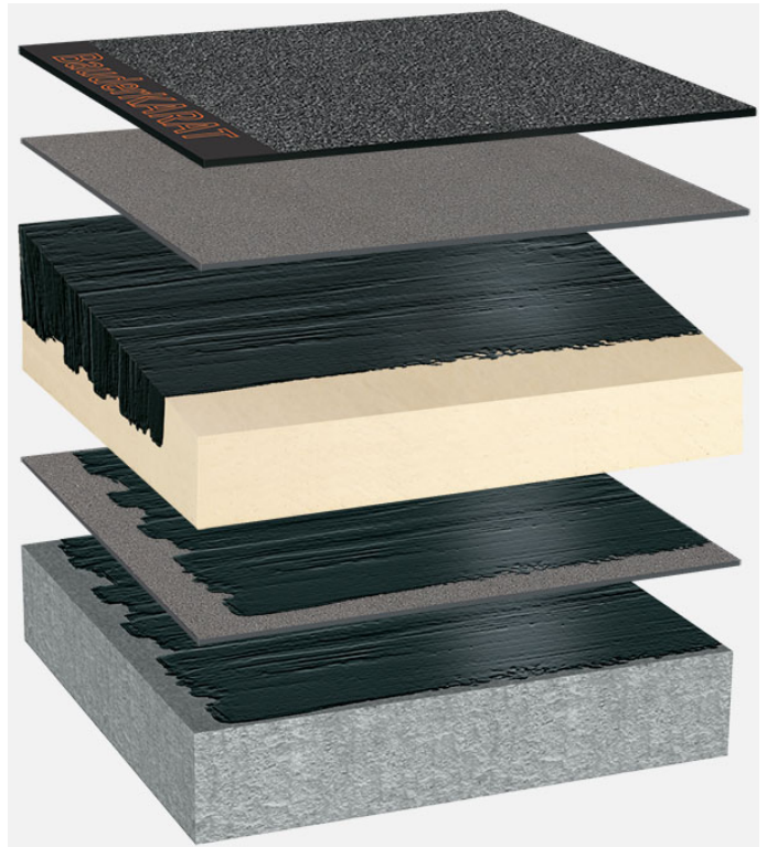
System oppbygging: BP_PIR-KG_K_01
