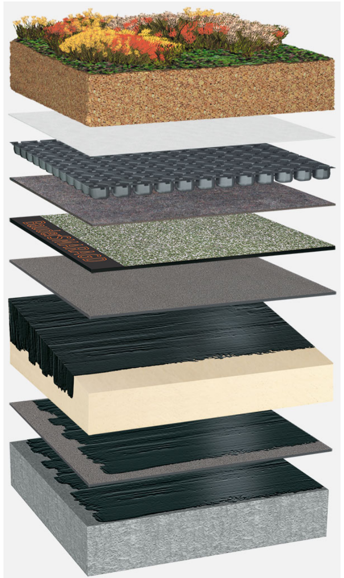
System oppbygging: BP_PIR-KG_S_01_G125
