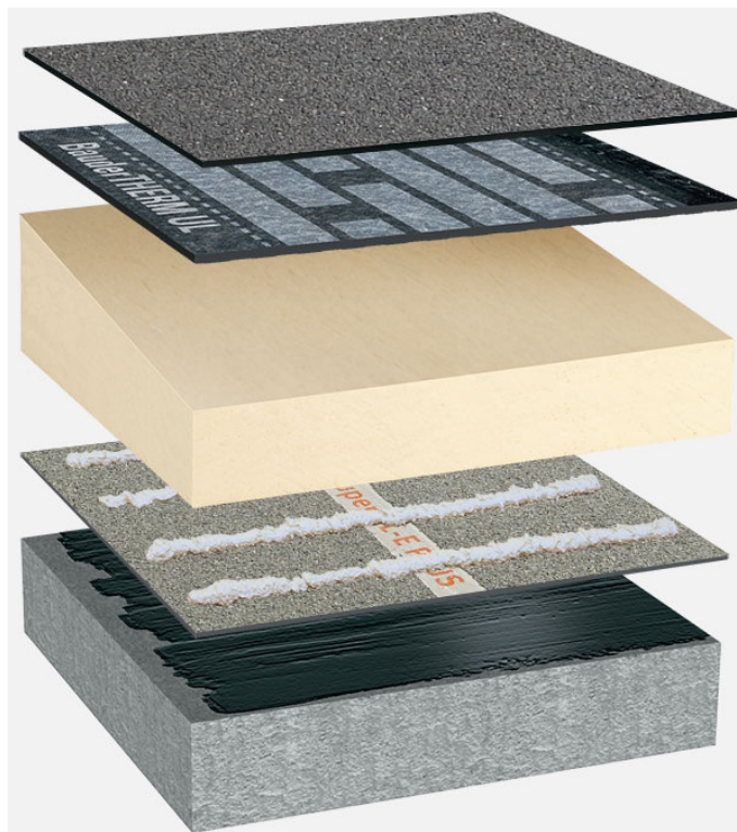
System oppbygging: BP_PIR-TG_B_01
