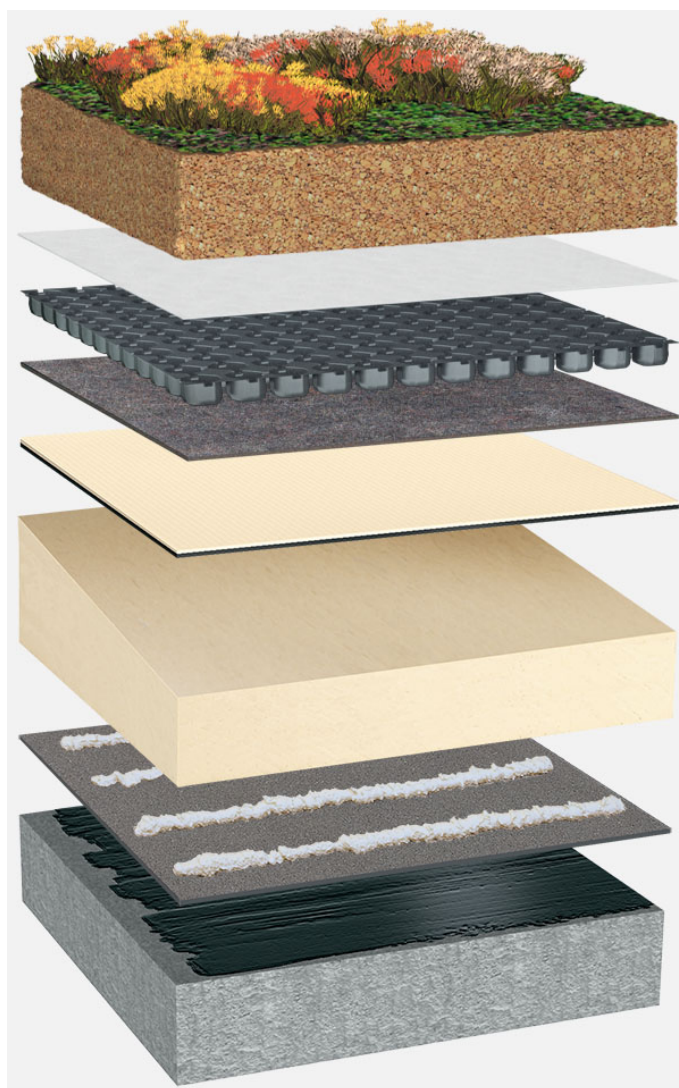
System oppbygging: BP_PIR-TG_T_01_G125
