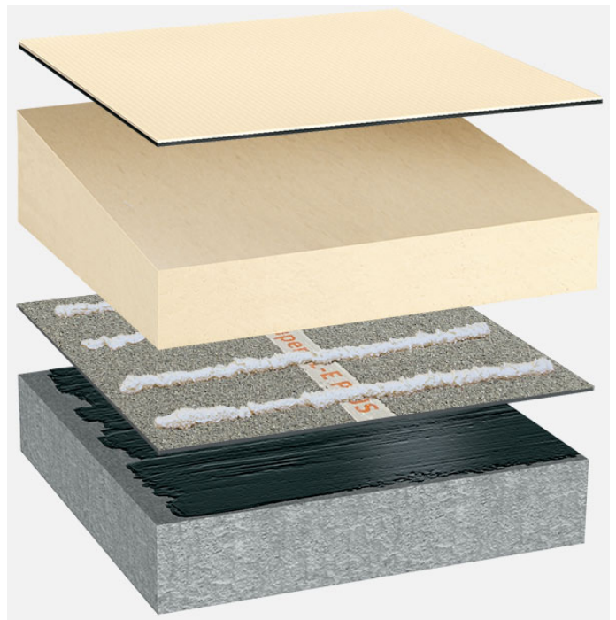
System oppbygging: BP_PIR-TG_T_02
